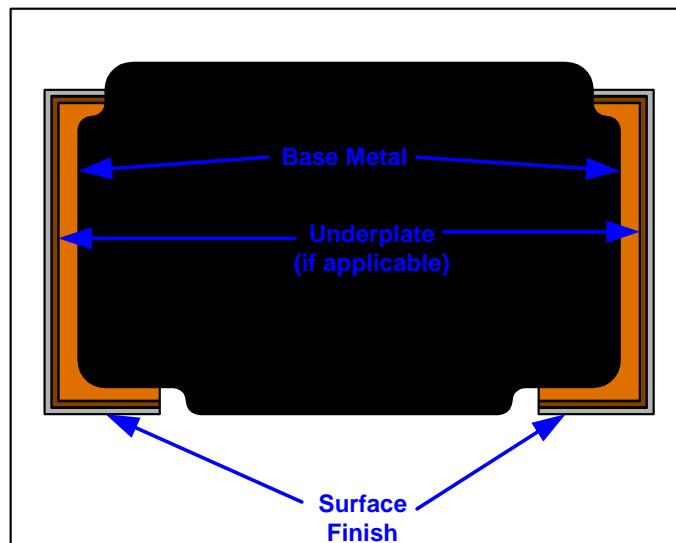
Figure 1 Cross-Sectional view of component surface finishes
