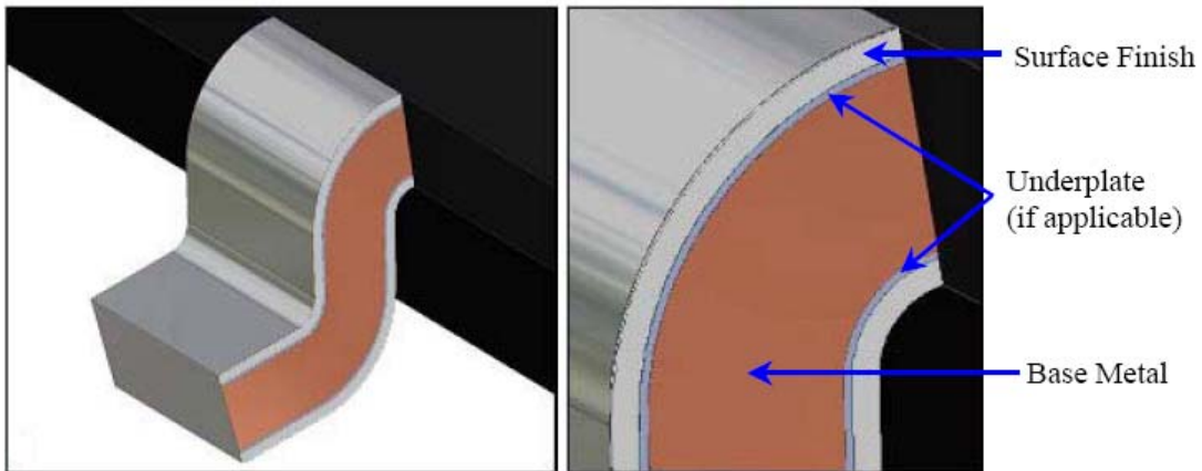
Figure 1 Cross-Sectional view of component surface finishes
