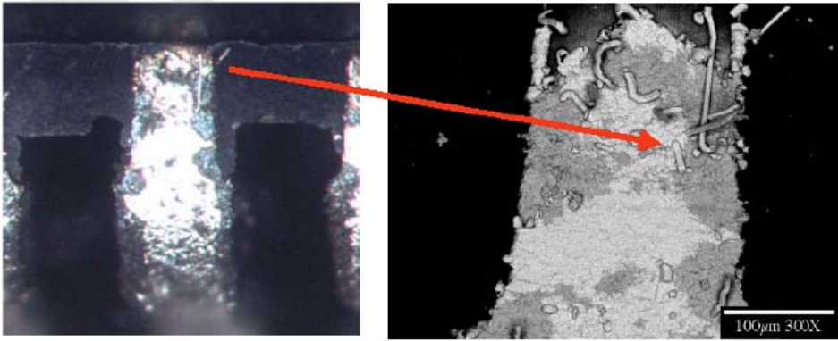
Matte Sn on Cu (Optical/SEM)
