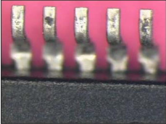
Matte Sn on Cu w/Nickel (optical)
